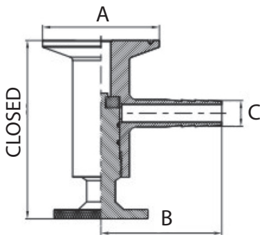
CLAMP STYLE
