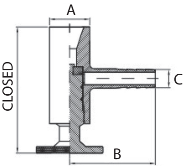
WELD STYLE
