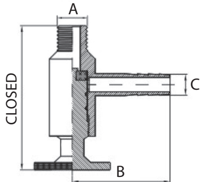
NPT STYLE
