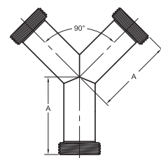
28B THREADED TRUE WYE
