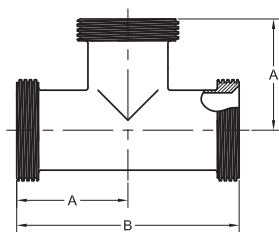
7 THREADED ENDS EQUAL TEE
